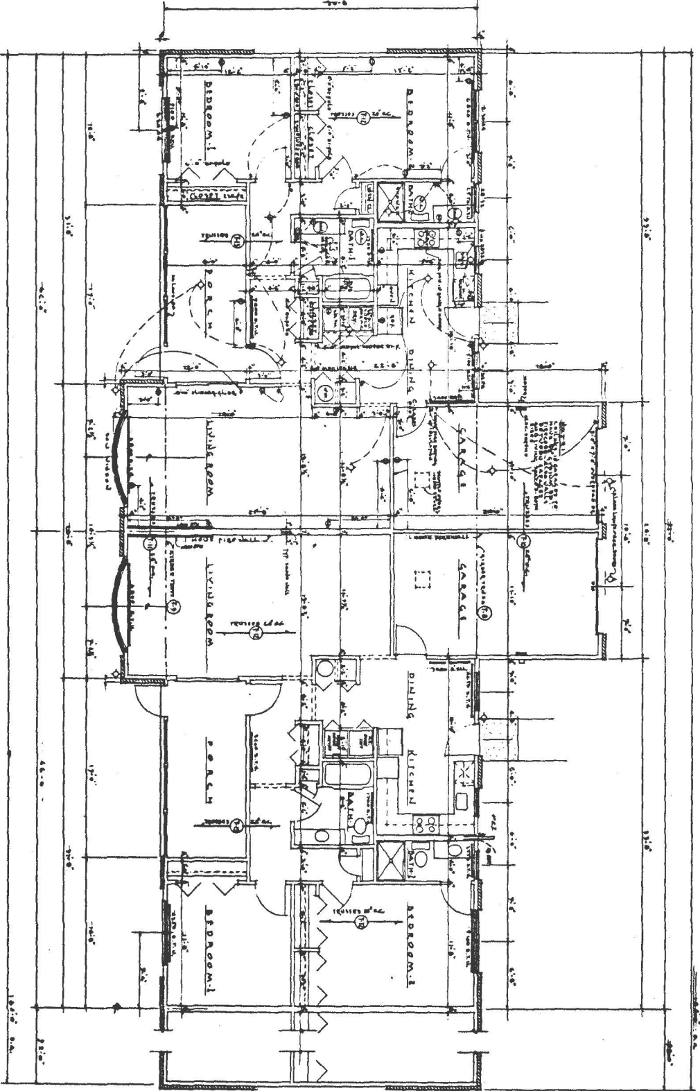
FLOOR PLAN VIEW NEW ATLAS APARTS BUILDING
