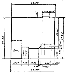
FRONT OF BLDG. TYPE 40
