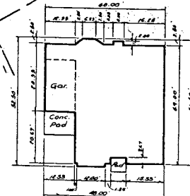
FRONT OF BLDG. TYPE 60
