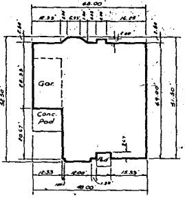
FRONT OF BLDG. TYPE 60
