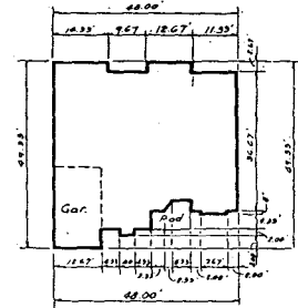
FRONT OF BLDG. TYPE 50
